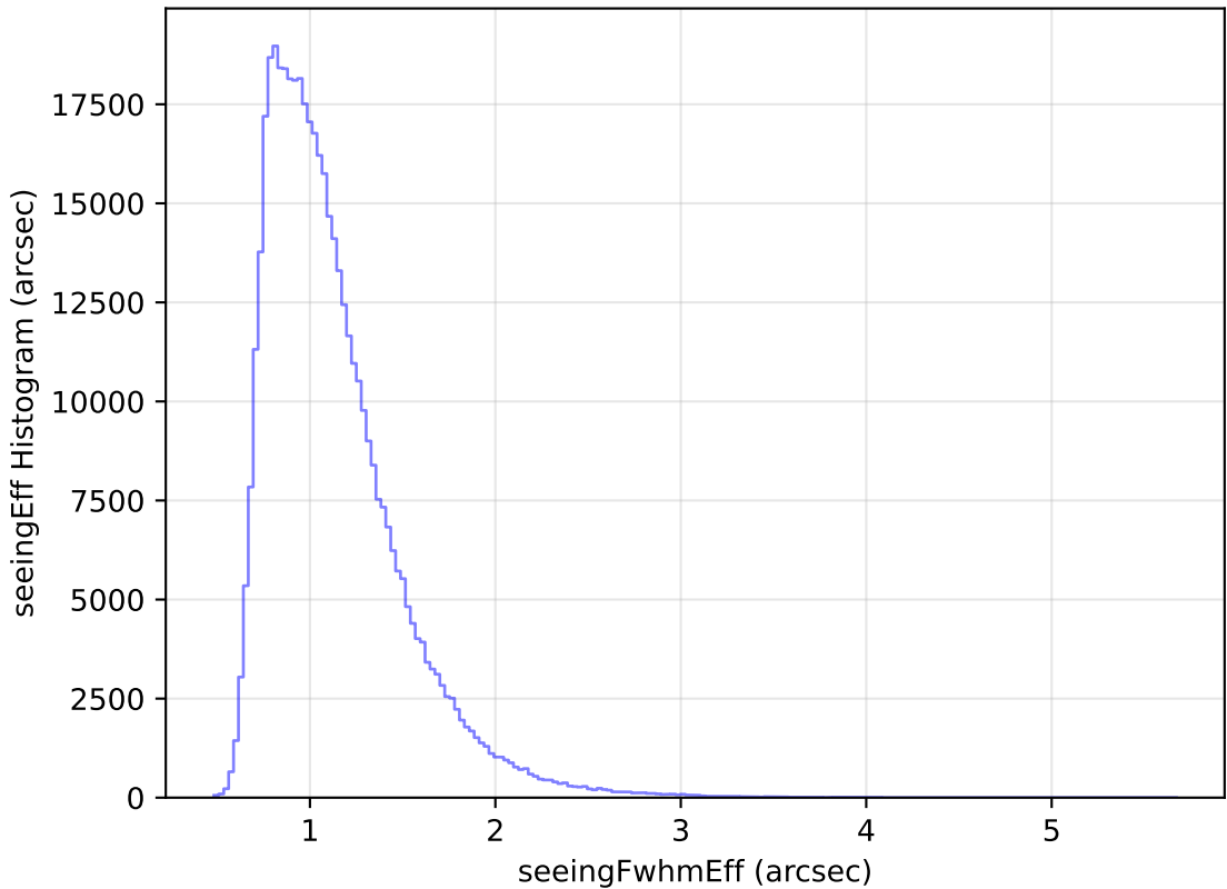
too_ignore_10_1v3.4_10yrs All sky r band: seeingEff Histogram
