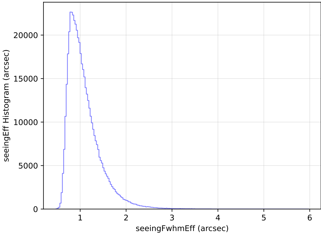
too_ignore_10_1v3.4_10yrs All sky i band: seeingEff Histogram
