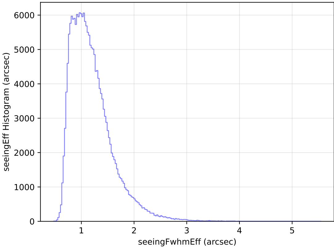
too_ignore_10_1v3.4_10yrs All sky g band: seeingEff Histogram
