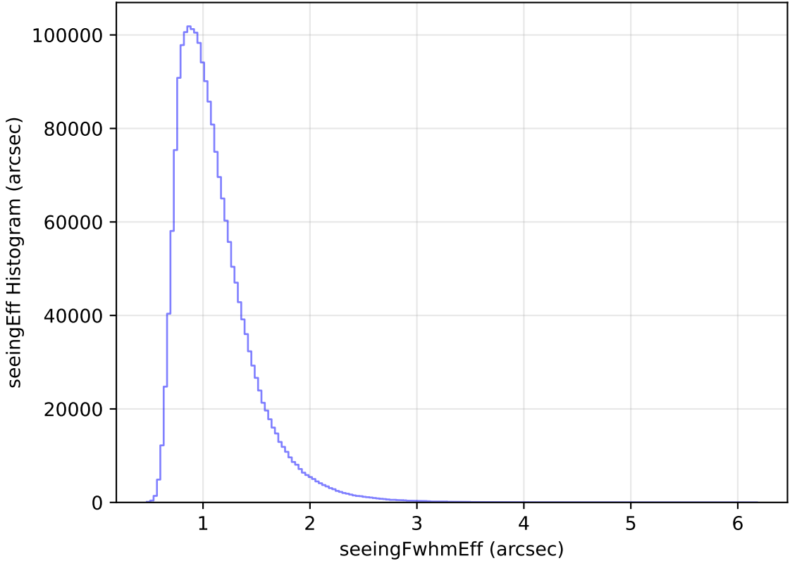
too_ignore_10_1v3.4_10yrs All sky all bands: seeingEff Histogram
