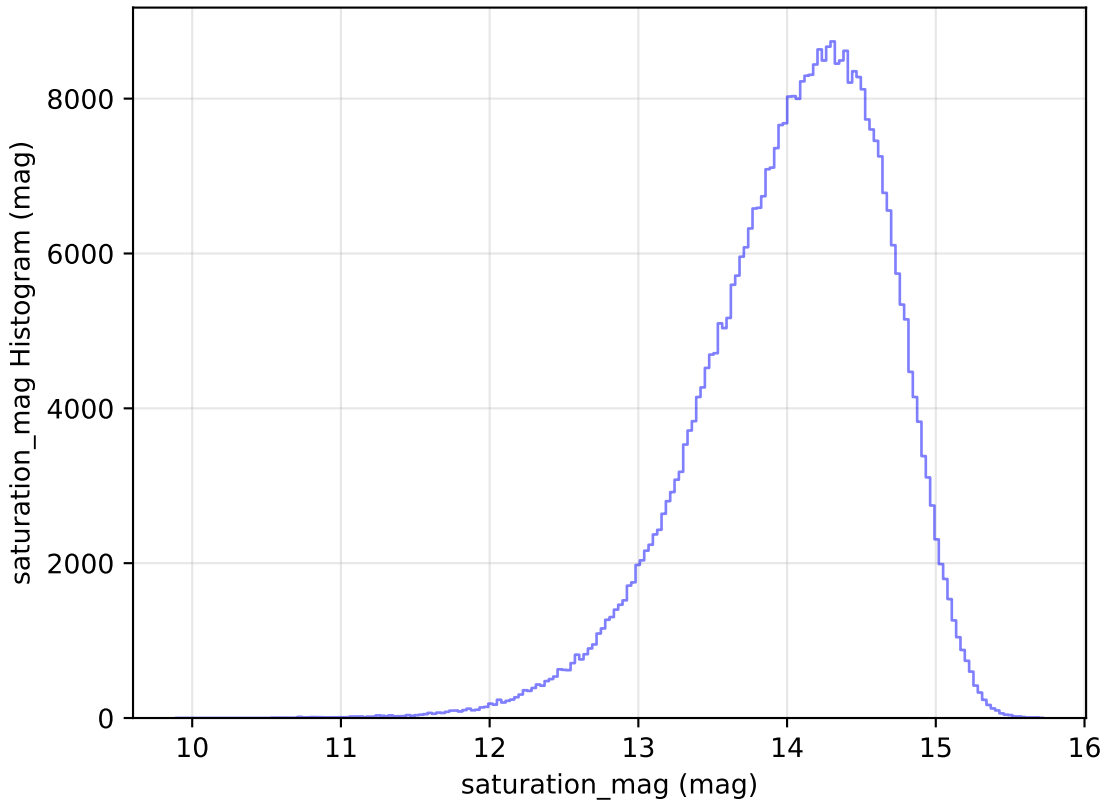
too_ignore_10_1v3.4_10yrs WFD z band: saturation_mag Histogram
