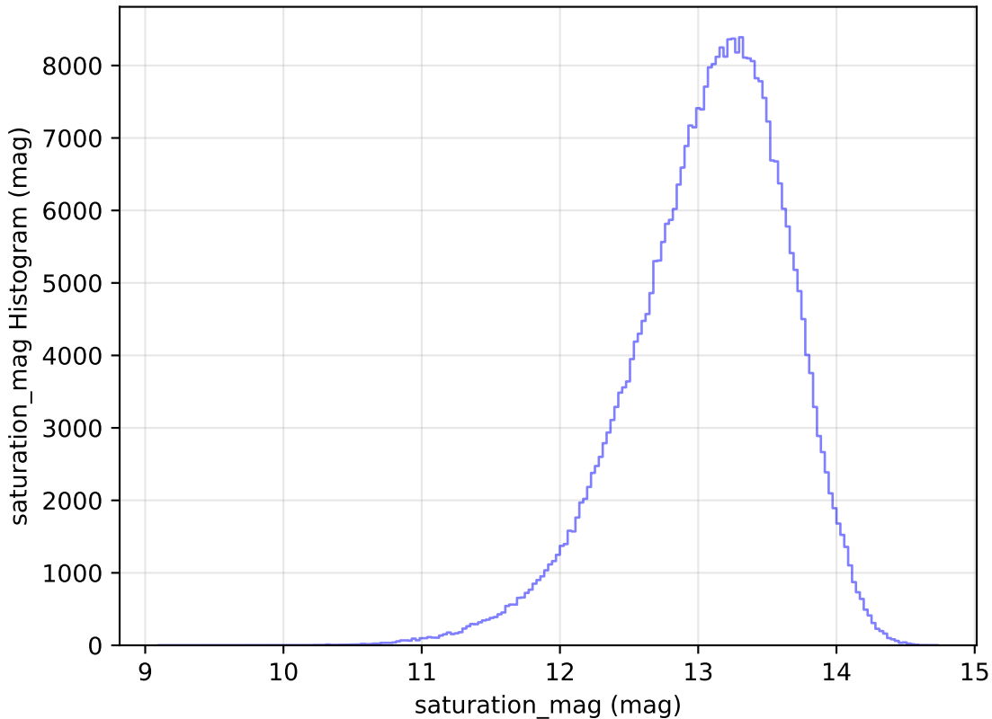
too_ignore_10_1v3.4_10yrs WFD y band: saturation_mag Histogram
