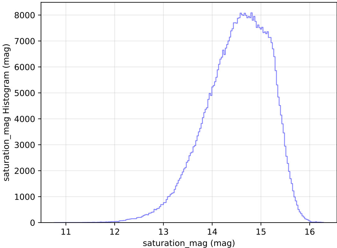
too_ignore_10_1v3.4_10yrs WFD r band: saturation_mag Histogram
