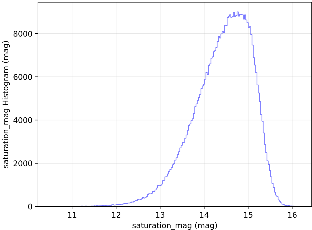
too_ignore_10_1v3.4_10yrs WFD i band: saturation_mag Histogram
