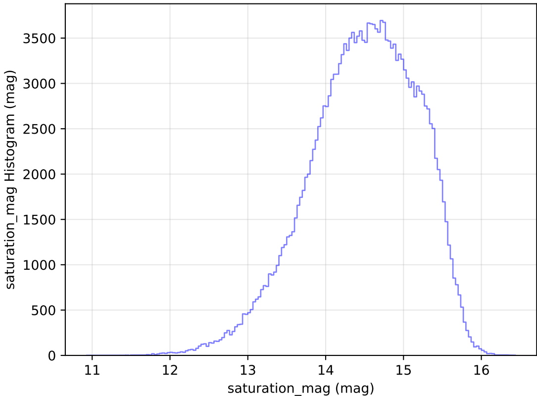
too_ignore_10_1v3.4_10yrs WFD g band: saturation_mag Histogram
