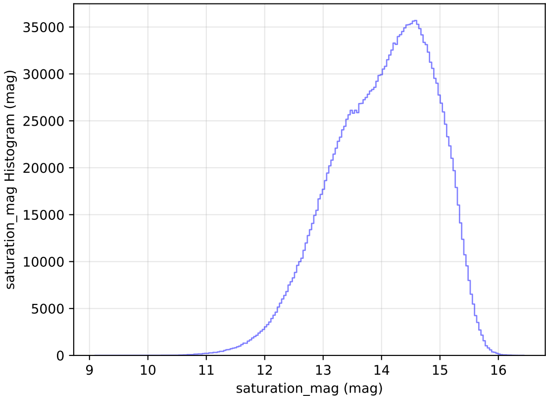
too_ignore_10_1v3.4_10yrs WFD all bands: saturation_mag Histogram
