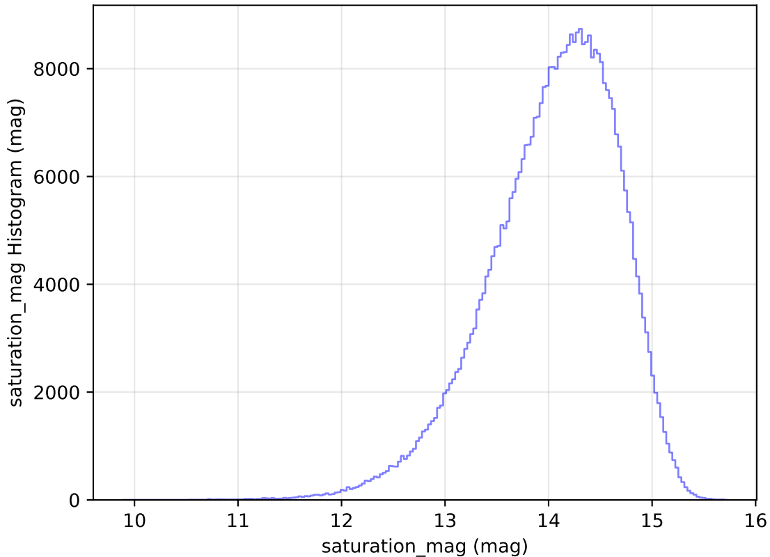
too_ignore_10_1v3.4_10yrs All sky z band: saturation_mag Histogram
