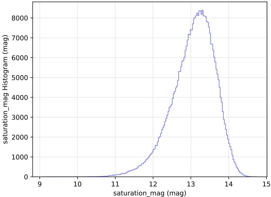
too_ignore_10_1v3.4_10yrs All sky y band: saturation_mag Histogram
