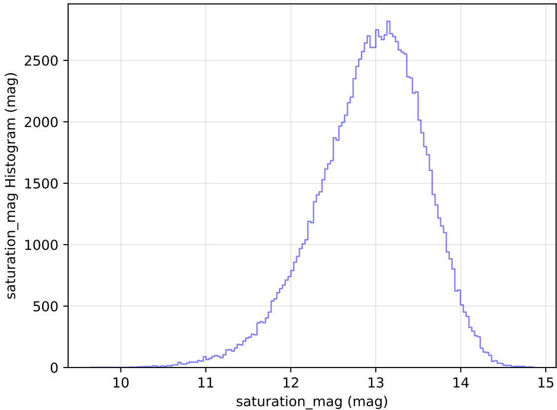
too_ignore_10_1v3.4_10yrs All sky u band: saturation_mag Histogram
