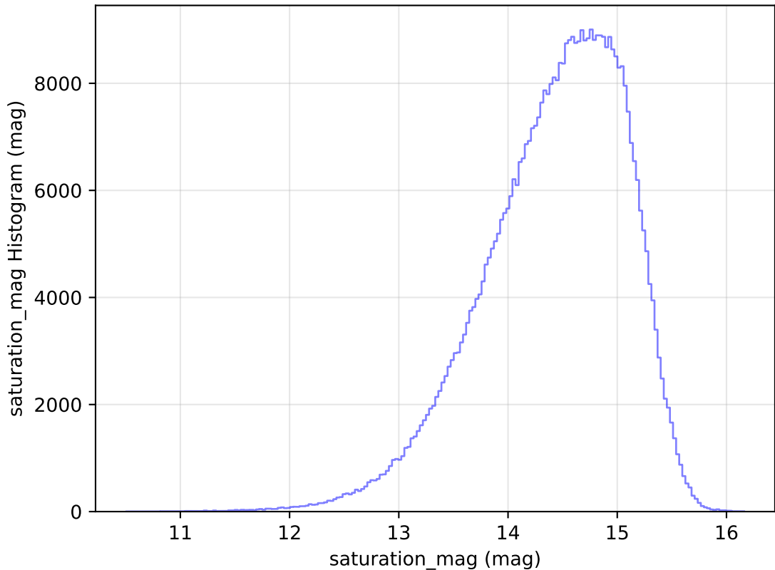
too_ignore_10_1v3.4_10yrs All sky i band: saturation_mag Histogram
