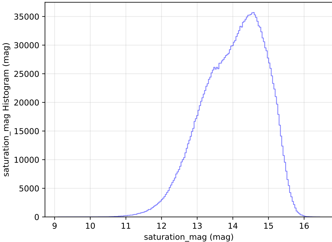
too_ignore_10_1v3.4_10yrs All sky all bands: saturation_mag Histogram
