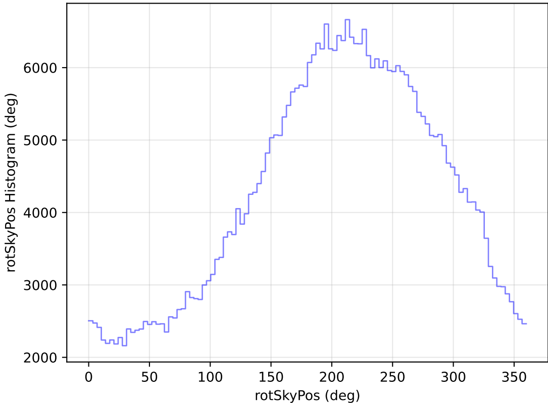
too_ignore_10_1v3.4_10yrs WFD z band: rotSkyPos Histogram
