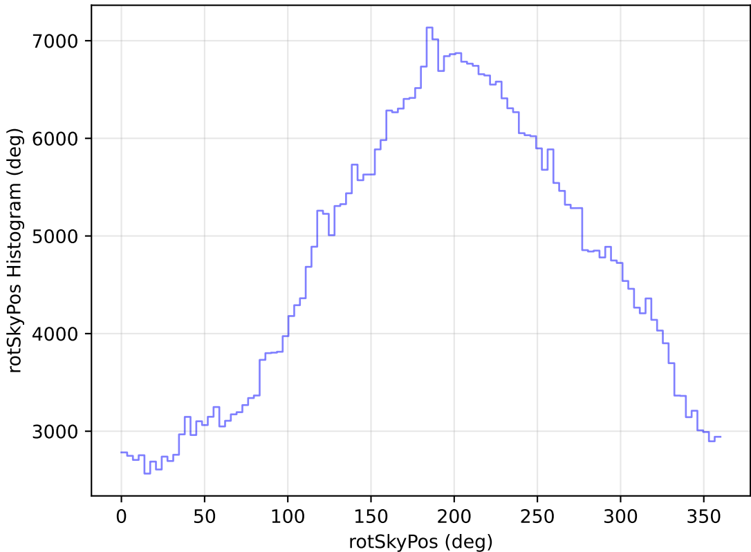
too_ignore_10_1v3.4_10yrs WFD r band: rotSkyPos Histogram
