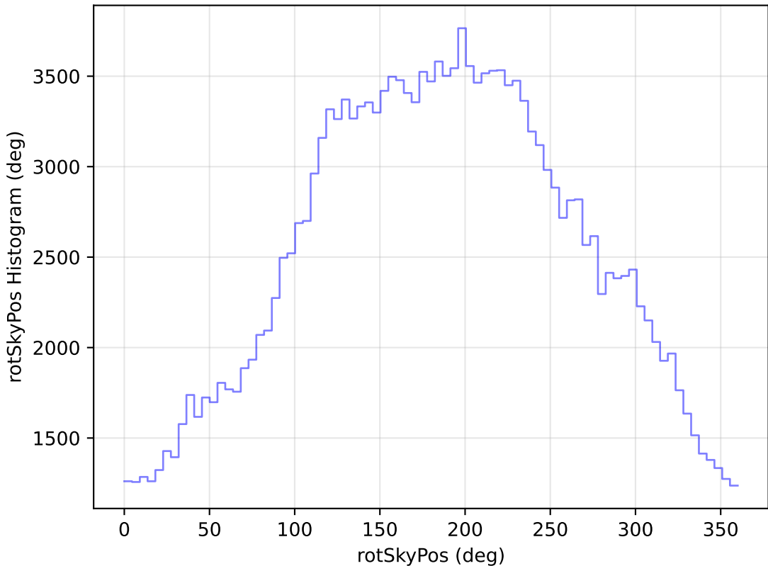
too_ignore_10_1v3.4_10yrs WFD g band: rotSkyPos Histogram
