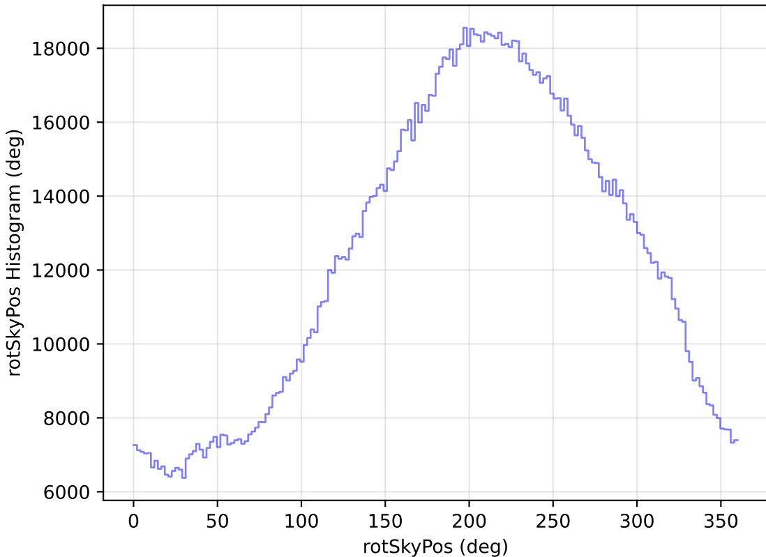
too_ignore_10_1v3.4_10yrs WFD all bands: rotSkyPos Histogram
