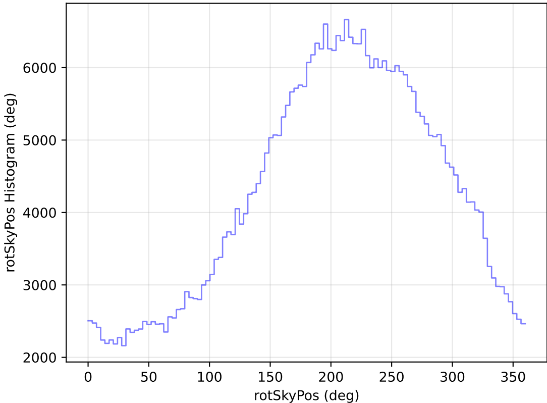
too_ignore_10_1v3.4_10yrs All sky z band: rotSkyPos Histogram
