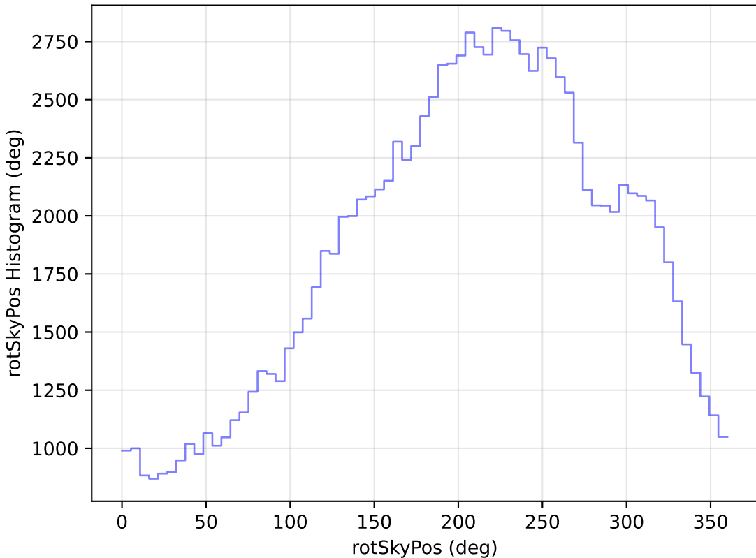
too_ignore_10_1v3.4_10yrs All sky u band: rotSkyPos Histogram
