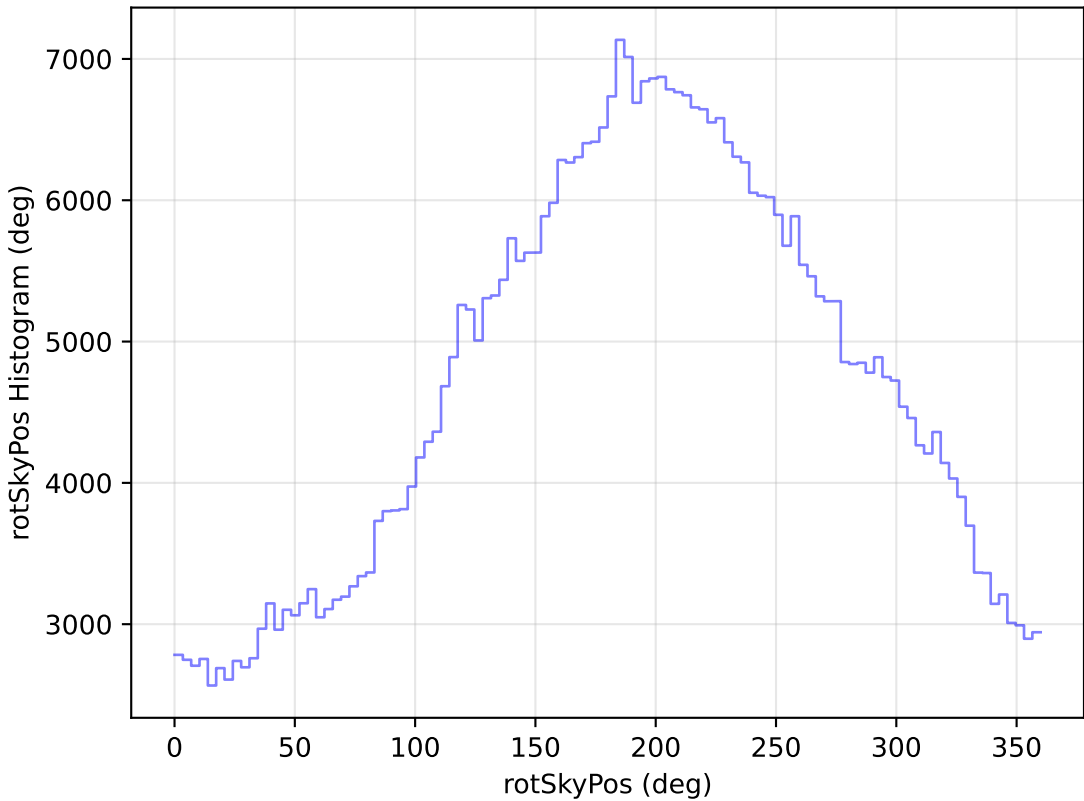
too_ignore_10_1v3.4_10yrs All sky r band: rotSkyPos Histogram
