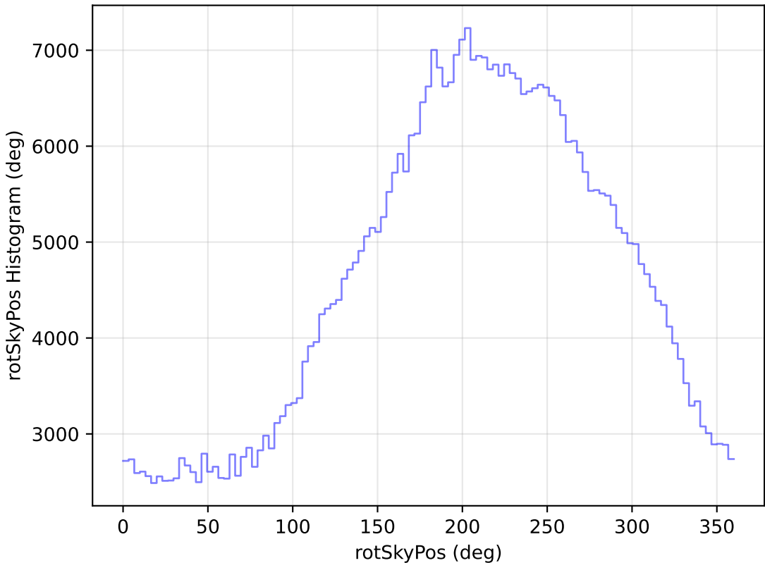
too_ignore_10_1v3.4_10yrs All sky i band: rotSkyPos Histogram
