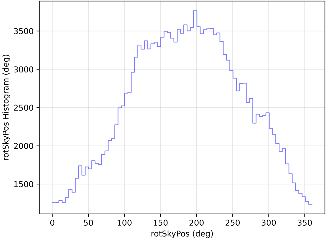
too_ignore_10_1v3.4_10yrs All sky g band: rotSkyPos Histogram
