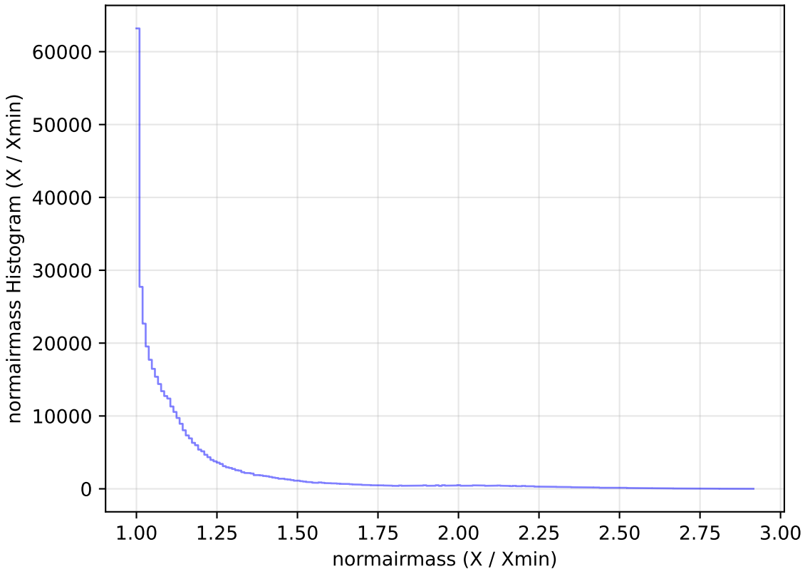
too_ignore_10_1v3.4_10yrs WFD z band: normairmass Histogram
