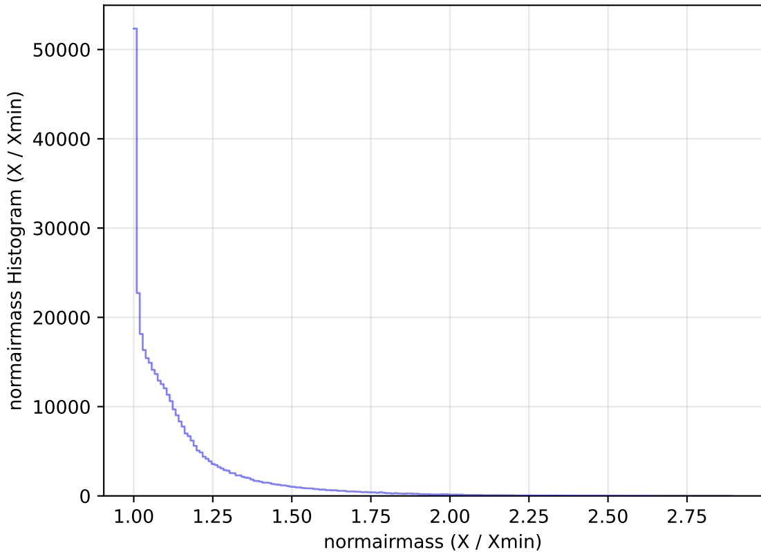
too_ignore_10_1v3.4_10yrs WFD y band: normairmass Histogram
