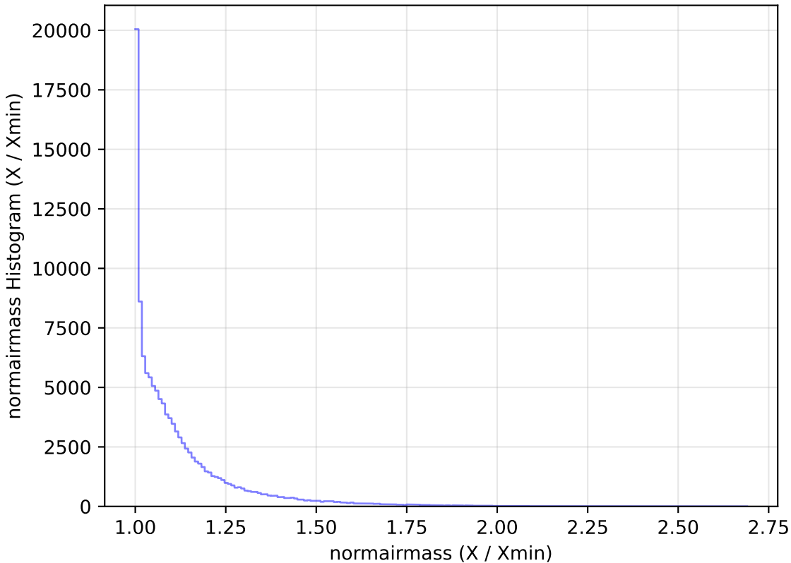
too_ignore_10_1v3.4_10yrs WFD u band: normairmass Histogram
