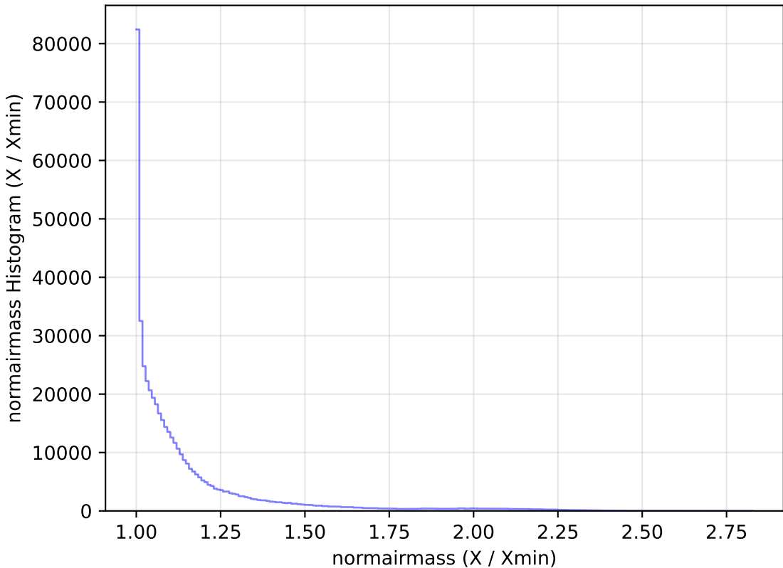
too_ignore_10_1v3.4_10yrs WFD r band: normairmass Histogram
