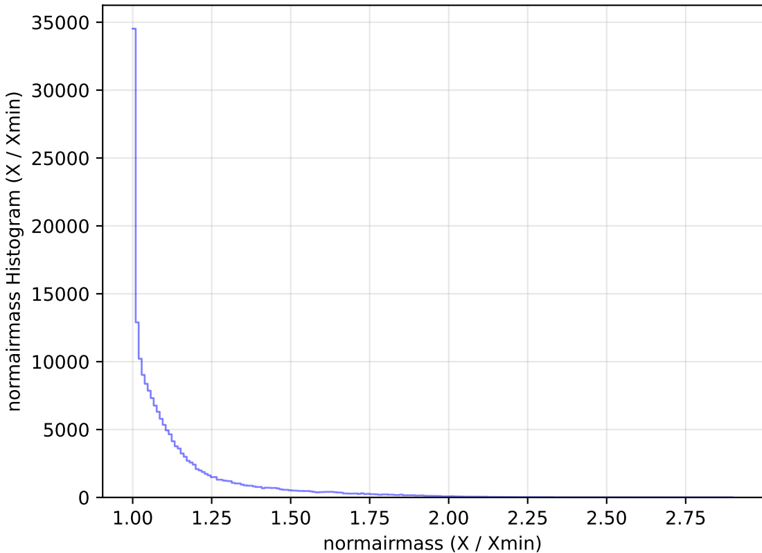
too_ignore_10_1v3.4_10yrs WFD g band: normairmass Histogram
