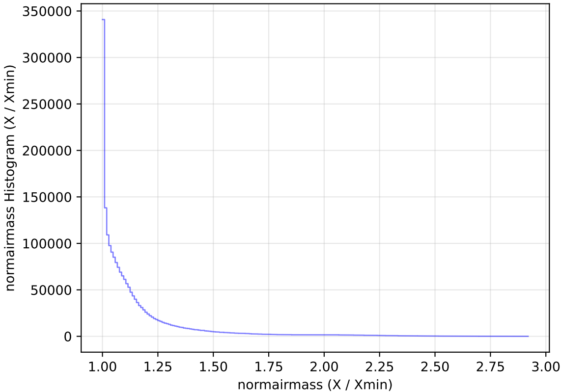
too_ignore_10_1v3.4_10yrs WFD all bands: normairmass Histogram
