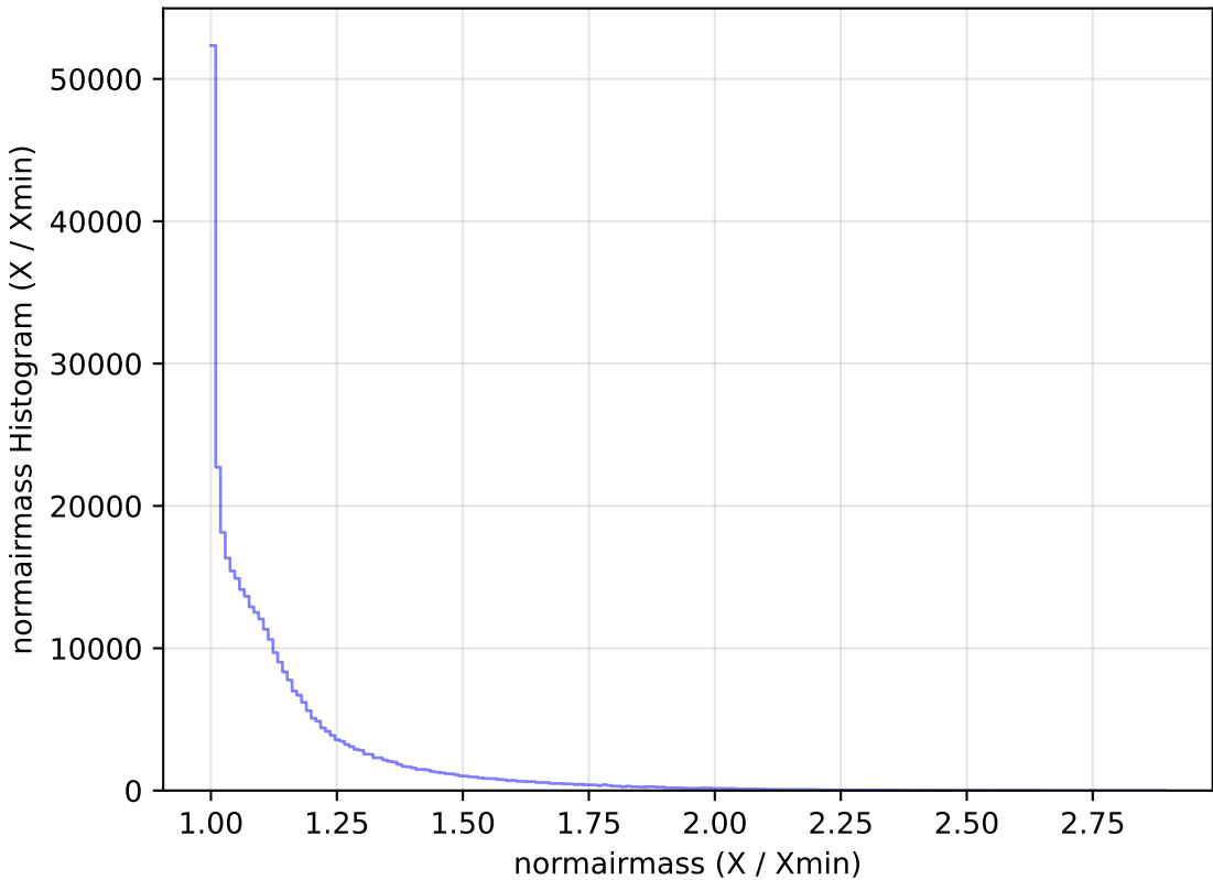
too_ignore_10_1v3.4_10yrs All sky y band: normairmass Histogram
