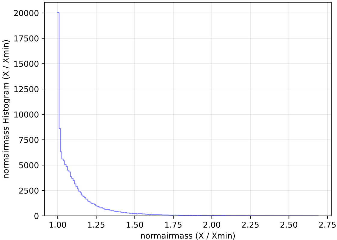
too_ignore_10_1v3.4_10yrs All sky u band: normairmass Histogram
