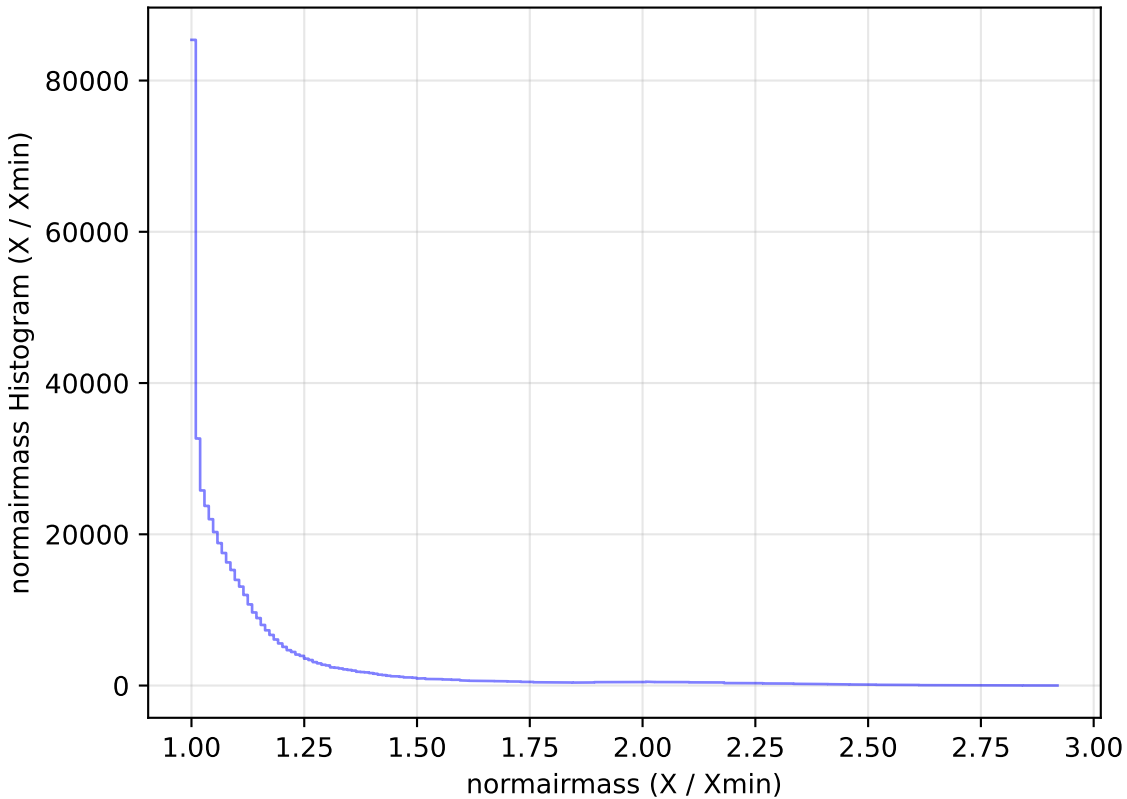
too_ignore_10_1v3.4_10yrs All sky i band: normairmass Histogram
