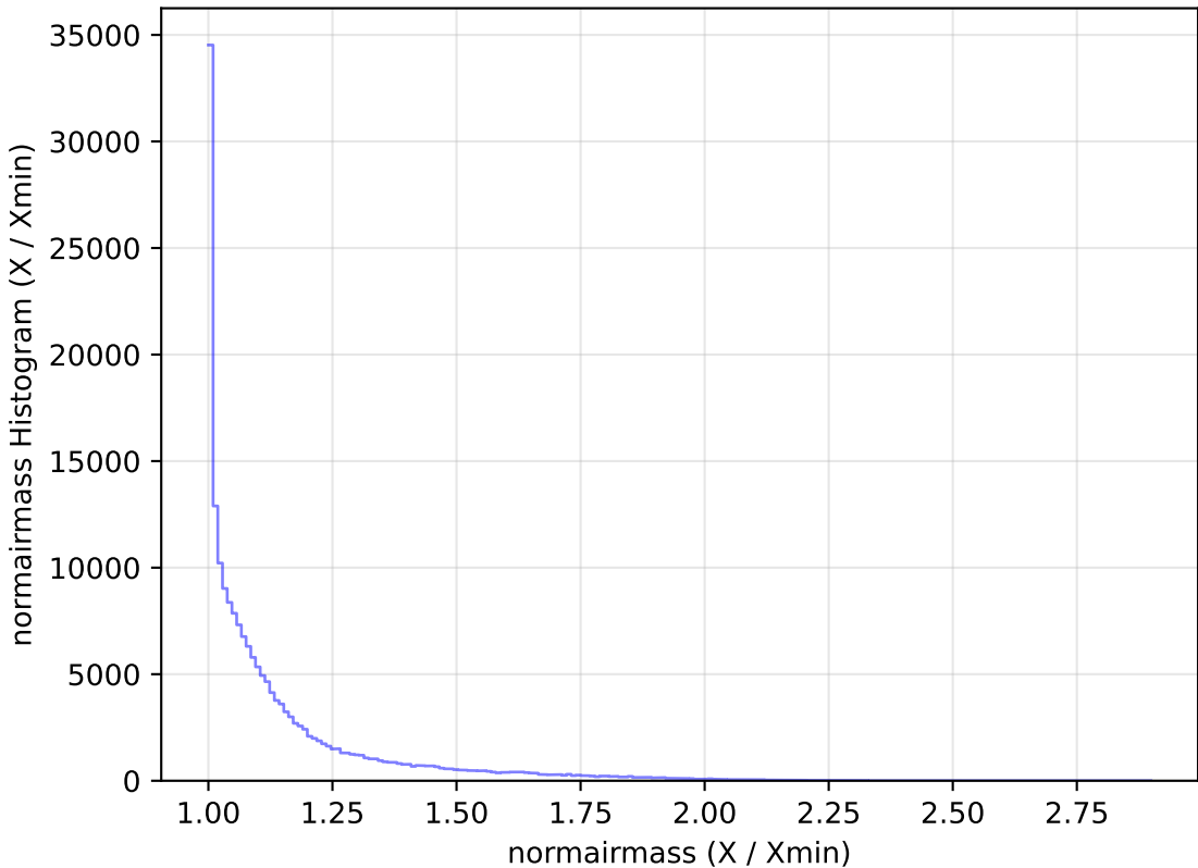
too_ignore_10_1v3.4_10yrs All sky g band: normairmass Histogram
