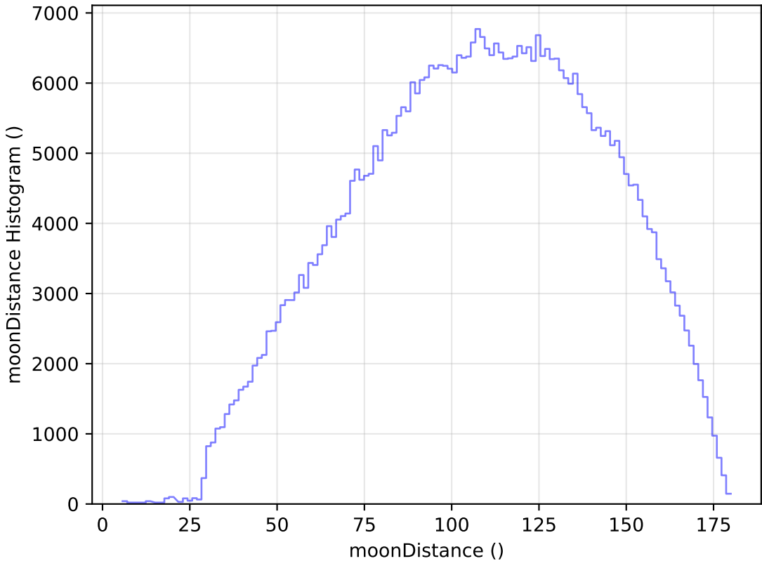
too_ignore_10_1v3.4_10yrs WFD r band: moonDistance Histogram
