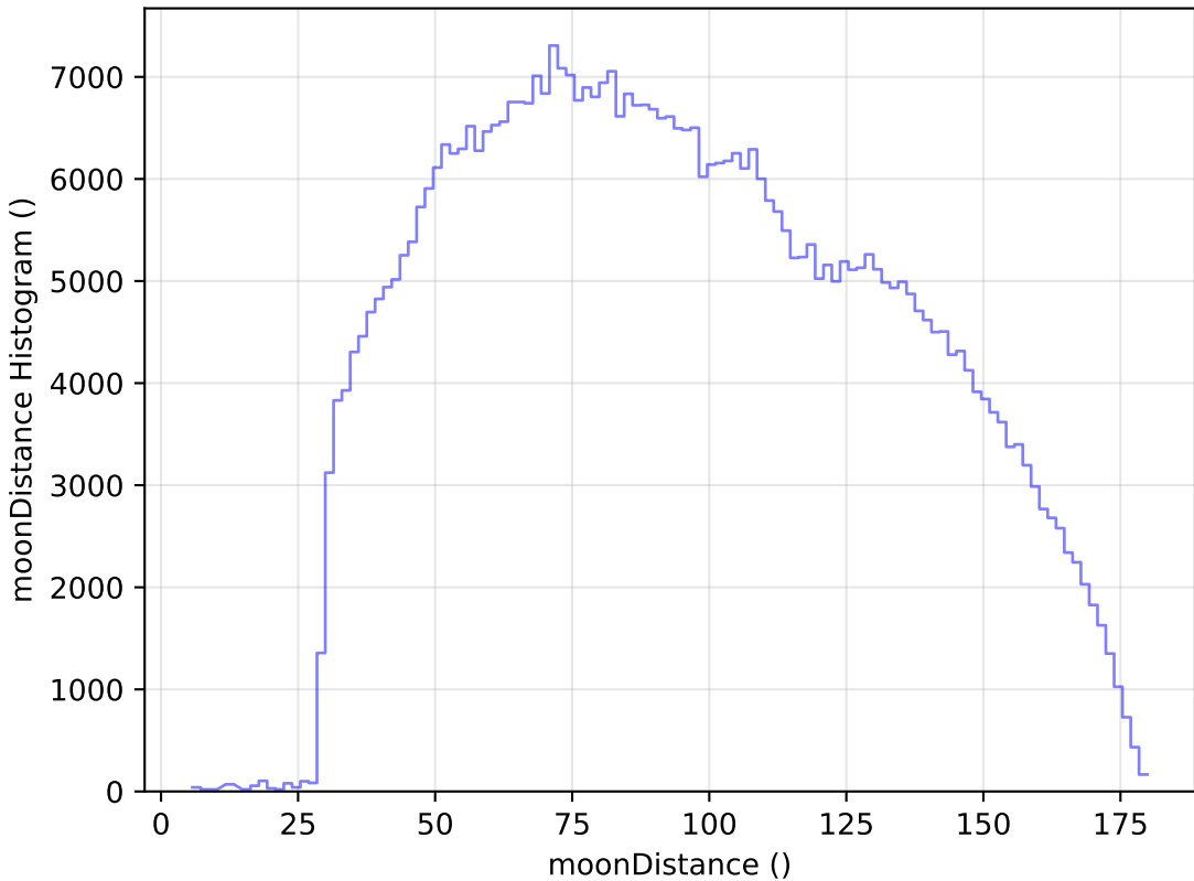
too_ignore_10_1v3.4_10yrs WFD i band: moonDistance Histogram
