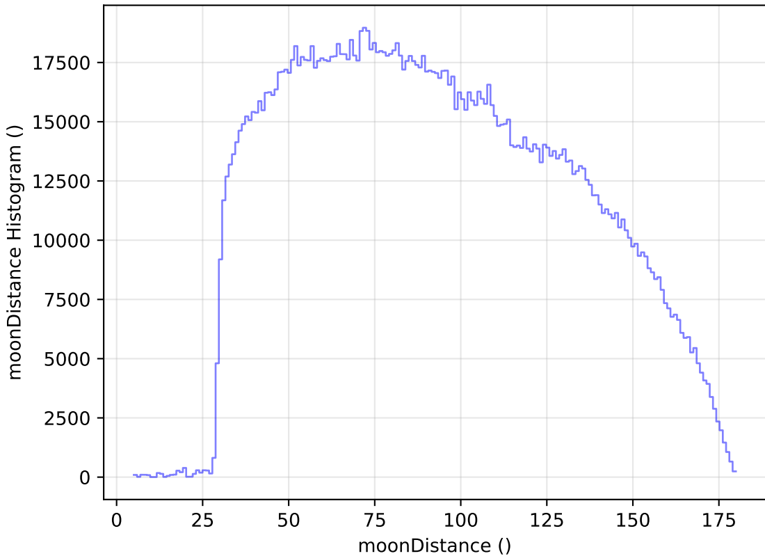
too_ignore_10_1v3.4_10yrs WFD all bands: moonDistance Histogram
