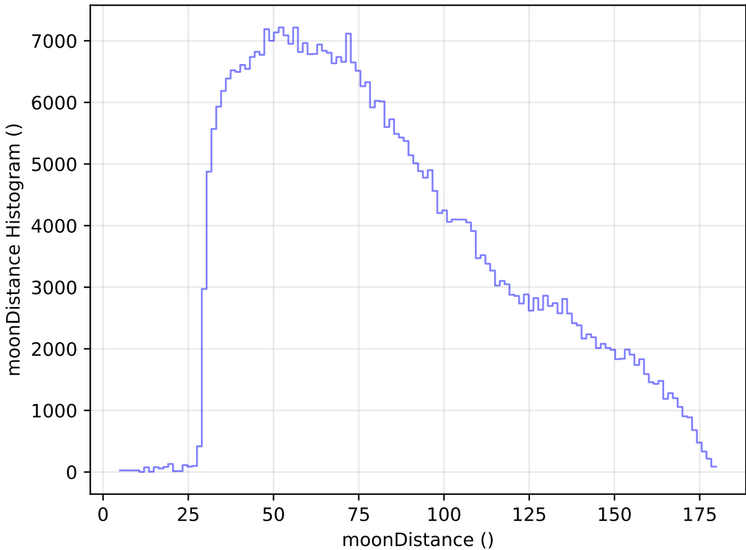
too_ignore_10_1v3.4_10yrs All sky z band: moonDistance Histogram
