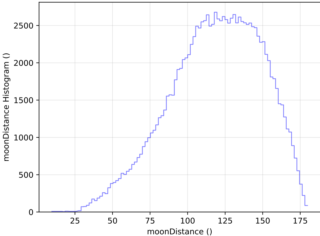
too_ignore_10_1v3.4_10yrs All sky u band: moonDistance Histogram
