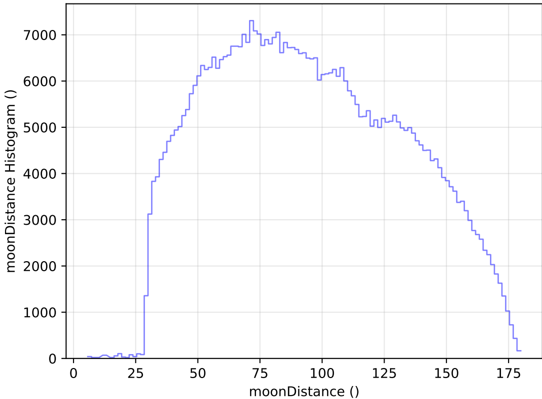
too_ignore_10_1v3.4_10yrs All sky i band: moonDistance Histogram
