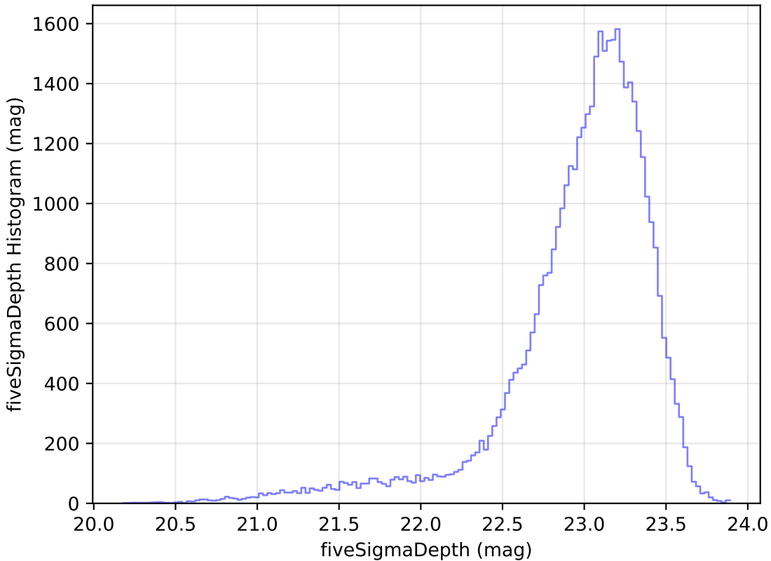
too_ignore_10_1v3.4_10yrs Yr 1 z band: fiveSigmaDepth Histogram
