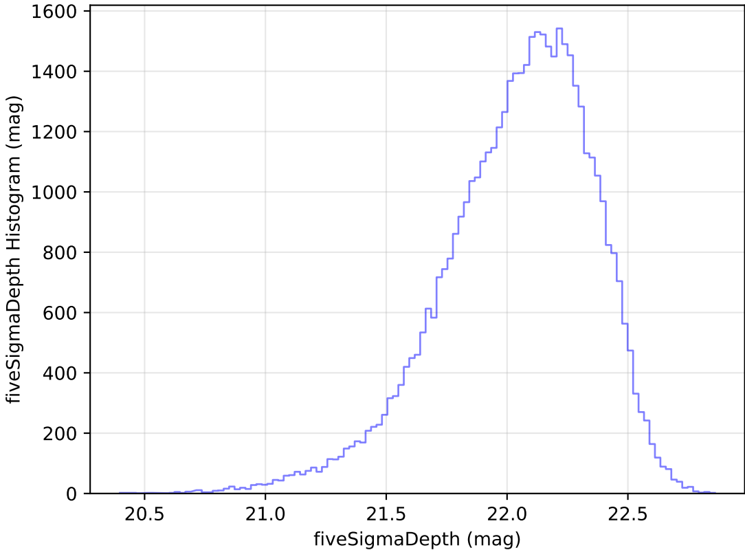
too_ignore_10_1v3.4_10yrs Yr 1 y band: fiveSigmaDepth Histogram
