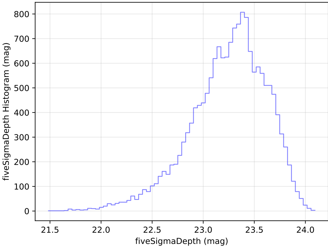
too_ignore_10_1v3.4_10yrs Yr 1 u band: fiveSigmaDepth Histogram
