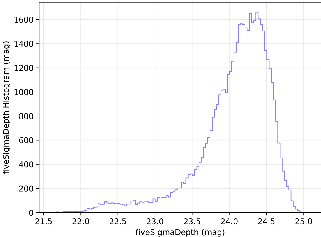
too_ignore_10_1v3.4_10yrs Yr 1 r band: fiveSigmaDepth Histogram
