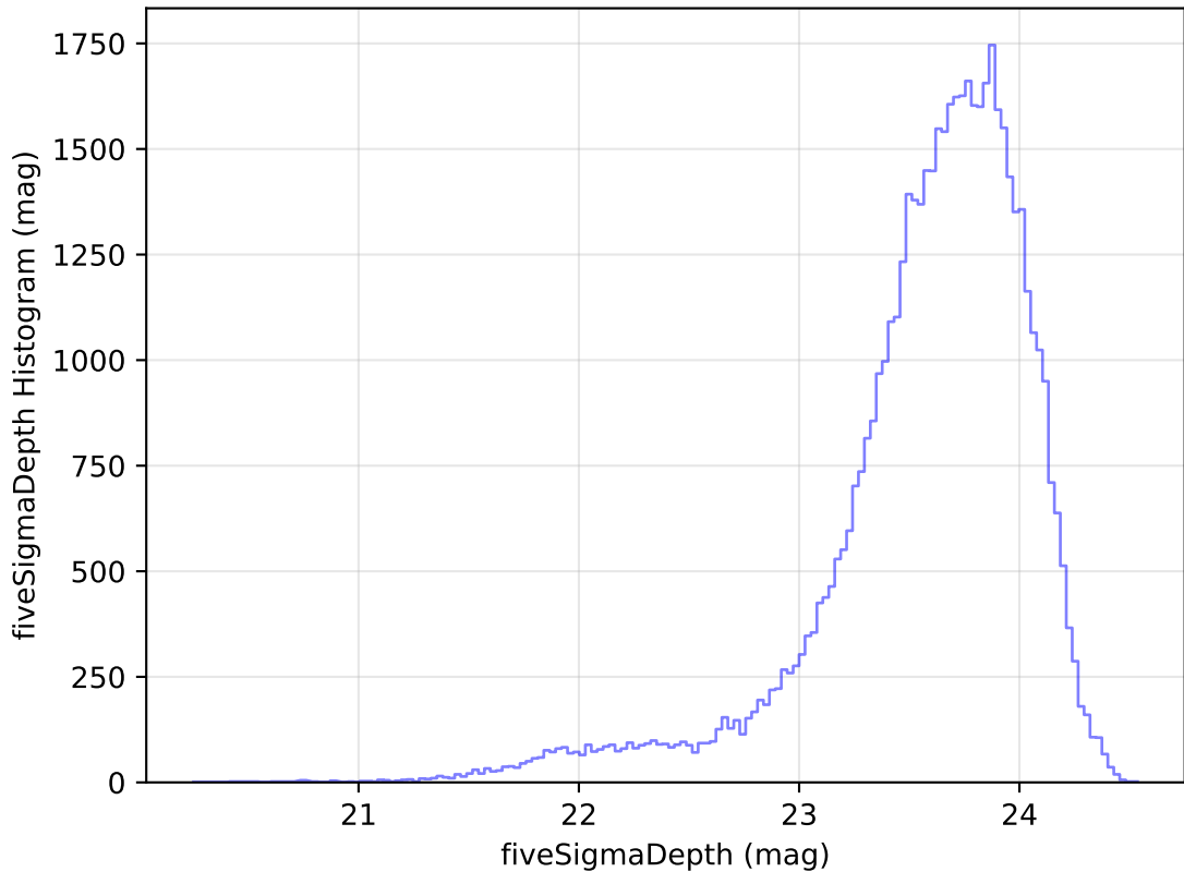
too_ignore_10_1v3.4_10yrs Yr 1 i band: fiveSigmaDepth Histogram
