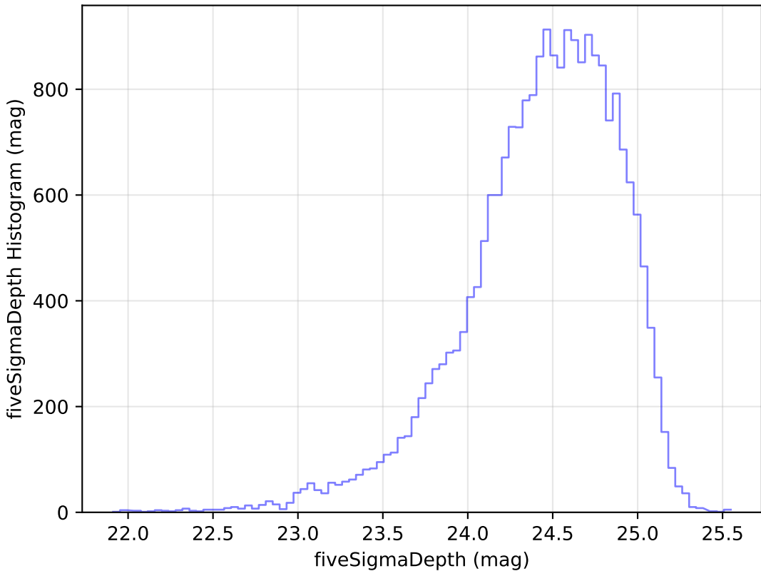
too_ignore_10_1v3.4_10yrs Yr 1 g band: fiveSigmaDepth Histogram
