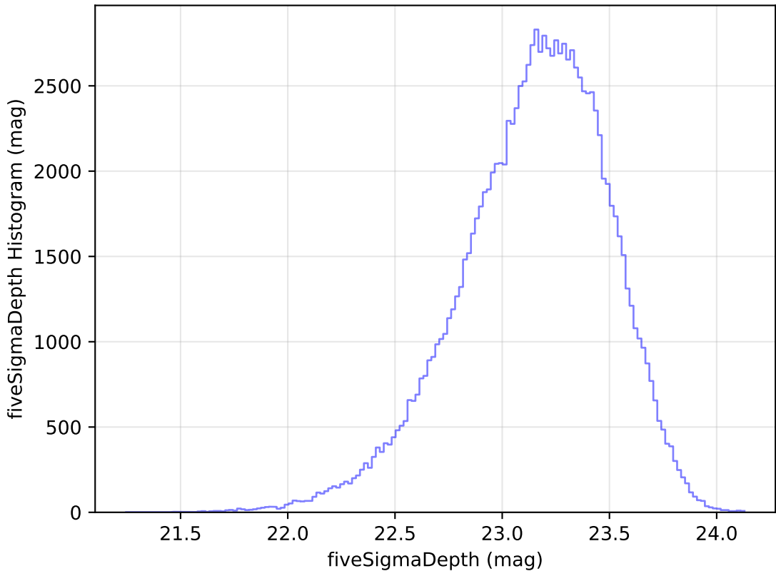
too_ignore_10_1v3.4_10yrs WFD u band: fiveSigmaDepth Histogram
