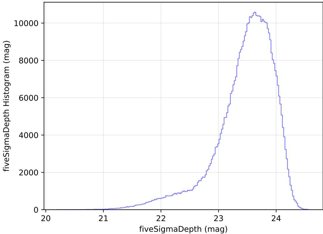
too_ignore_10_1v3.4_10yrs WFD i band: fiveSigmaDepth Histogram
