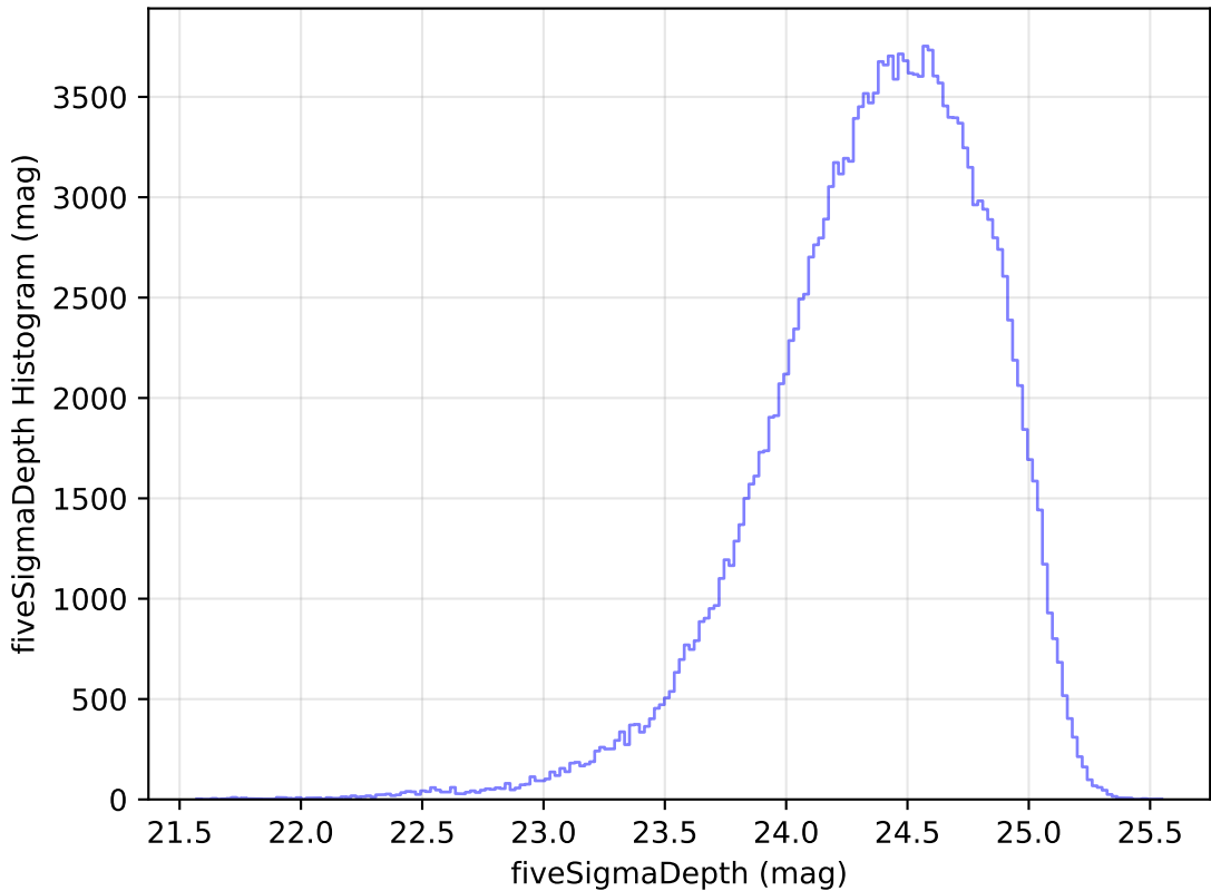
too_ignore_10_1v3.4_10yrs WFD g band: fiveSigmaDepth Histogram
