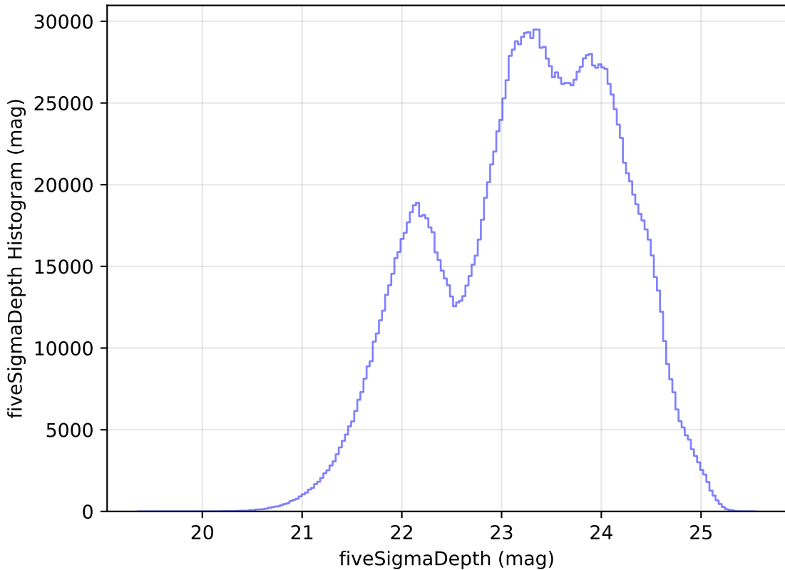
too_ignore_10_1v3.4_10yrs WFD all bands: fiveSigmaDepth Histogram
